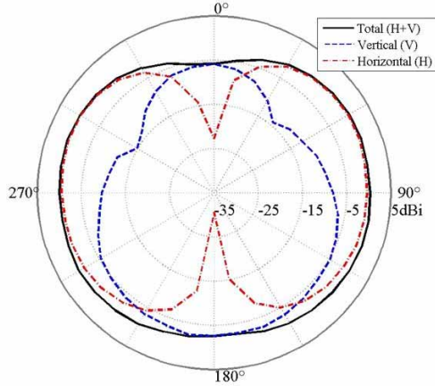
DCS ( f_c = 1795\text{MHz} )
