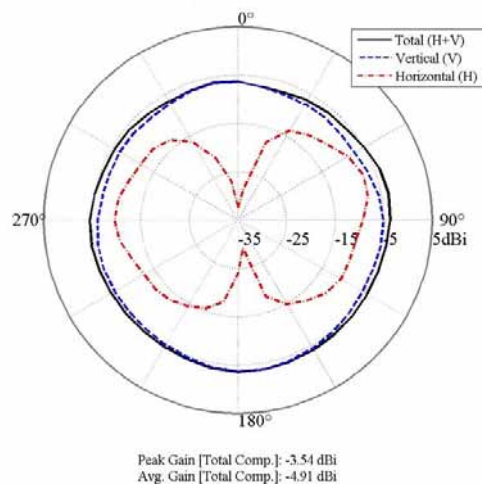
GSM900 ( f_c = 920\text{MHz} )
