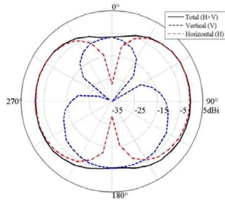
PCS ( f_c = 1920\text{MHz} )
