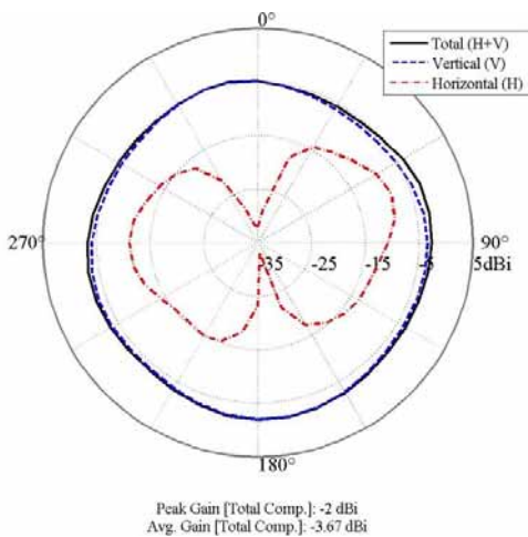
GSM850 ( f_c = 859\text{MHz} )
